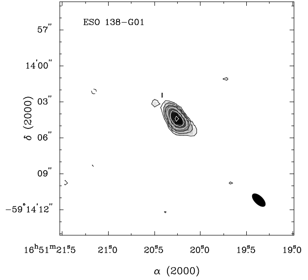
Fig. 11. ESO138-G01 Contours: -0.7, -0.4, 0.4, 0.7, 1.1, 1.6, 2.5, 3.9 mJy beam ^{-1}
